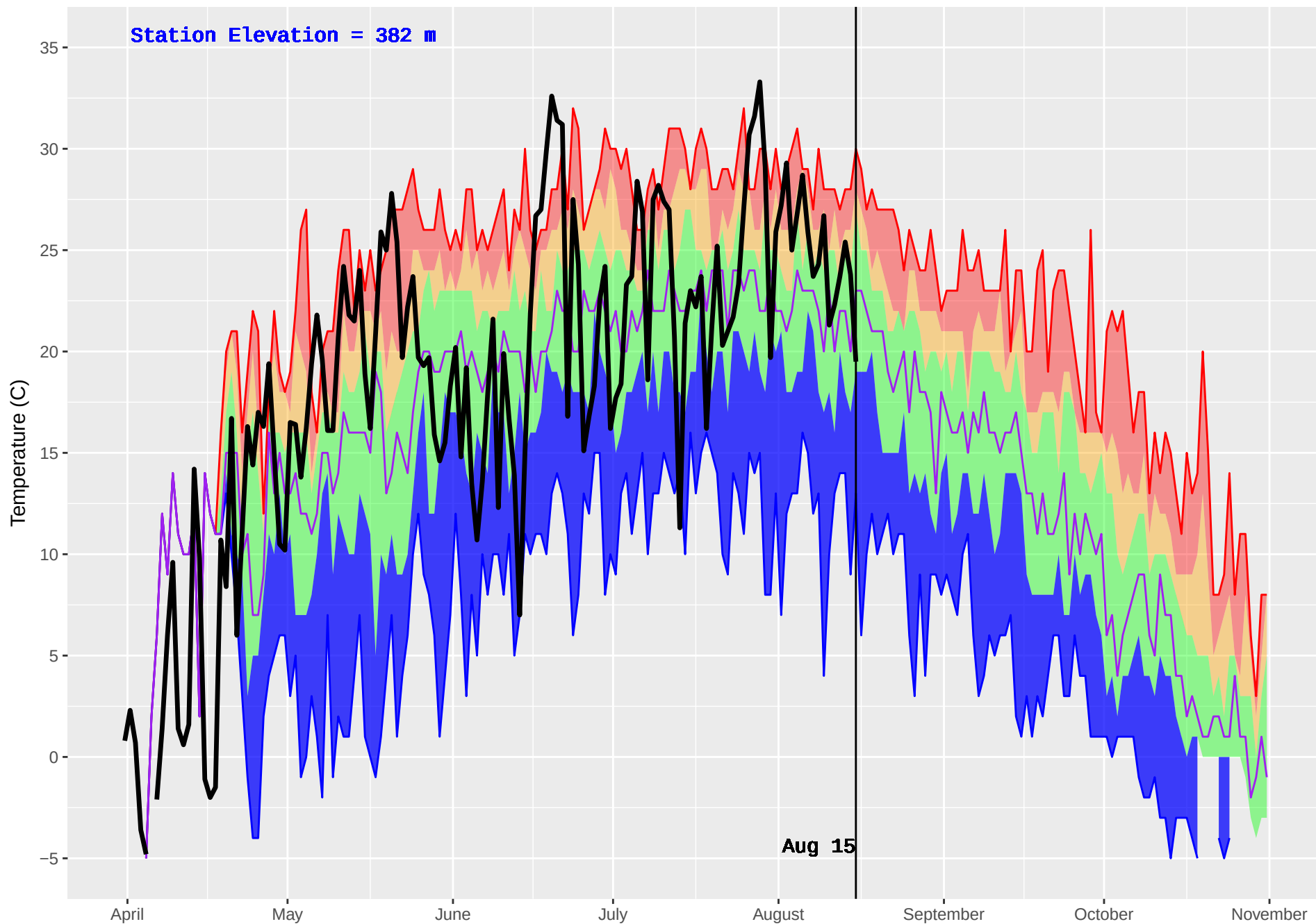
FORT NELSON FS (599) : Historical (1999–2016) and Current (2018) Daily Temperature
