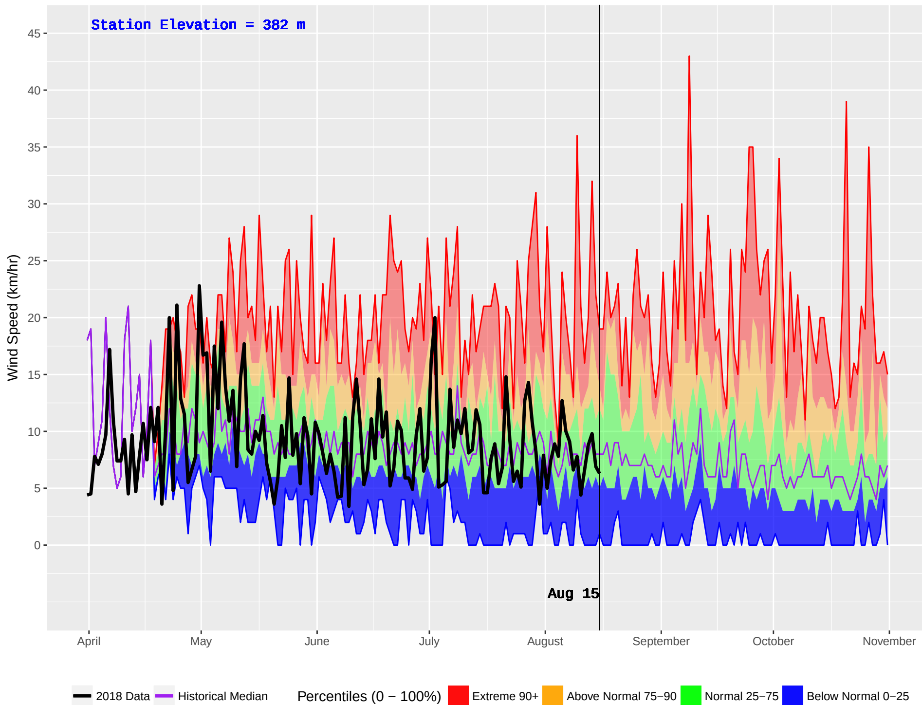
FORT NELSON FS (599) : Historical (1999–2016) and Current (2018) Daily Wind Speed
