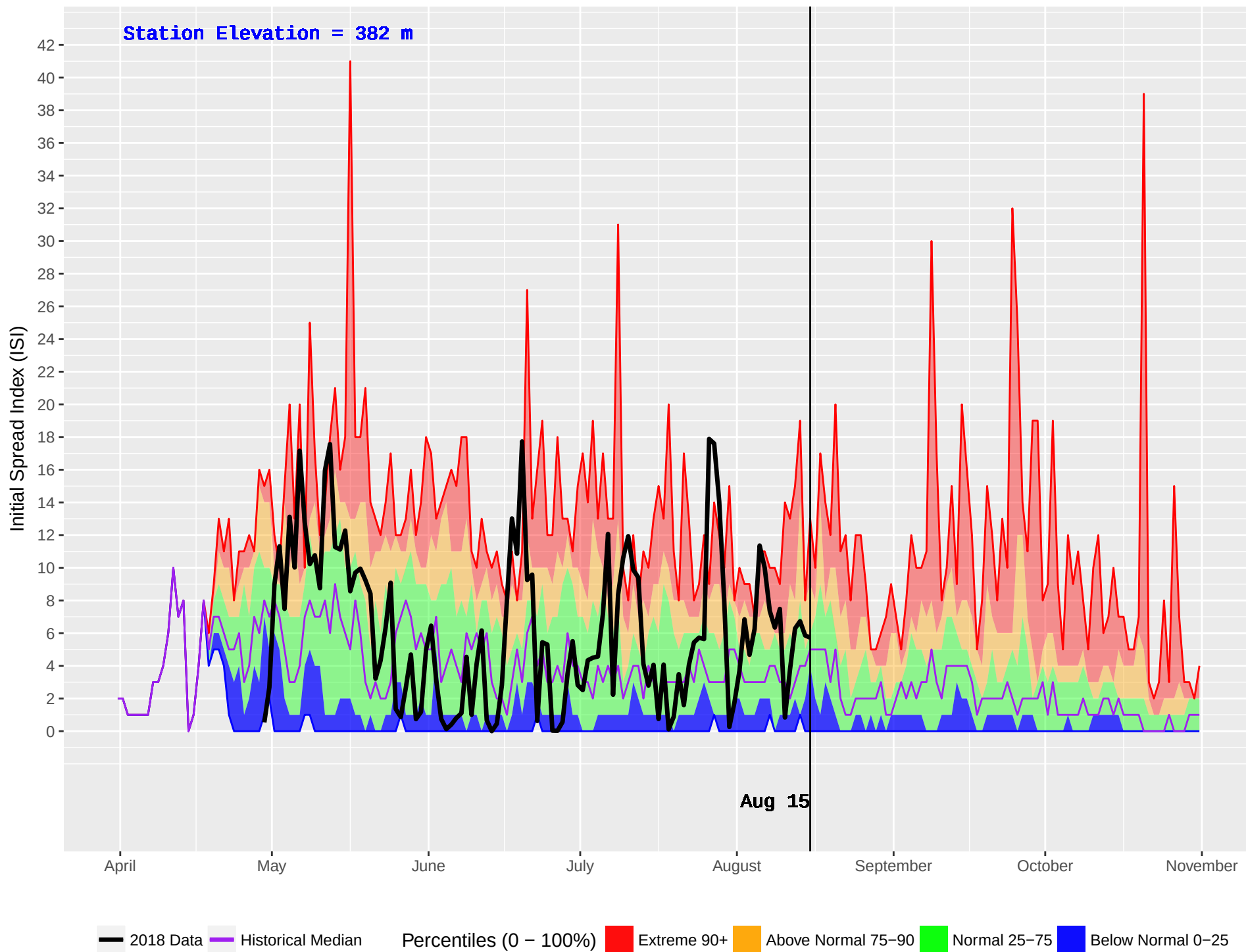
FORT NELSON FS (599) : Historical (1999–2016) and Current (2018) Daily Initial Spread Index (ISI)
