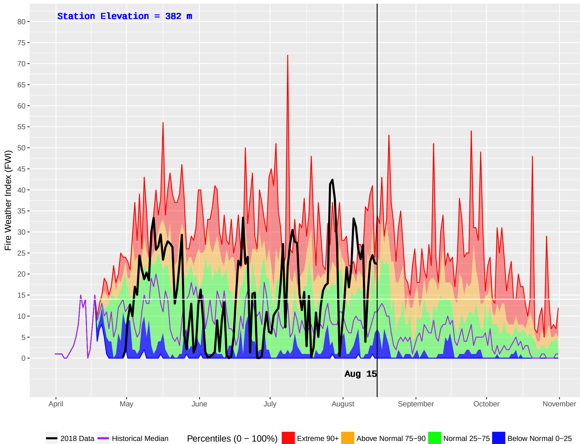
FORT NELSON FS (599) : Historical (1999–2016) and Current (2018) Daily Fire Weather Index (FWI)
