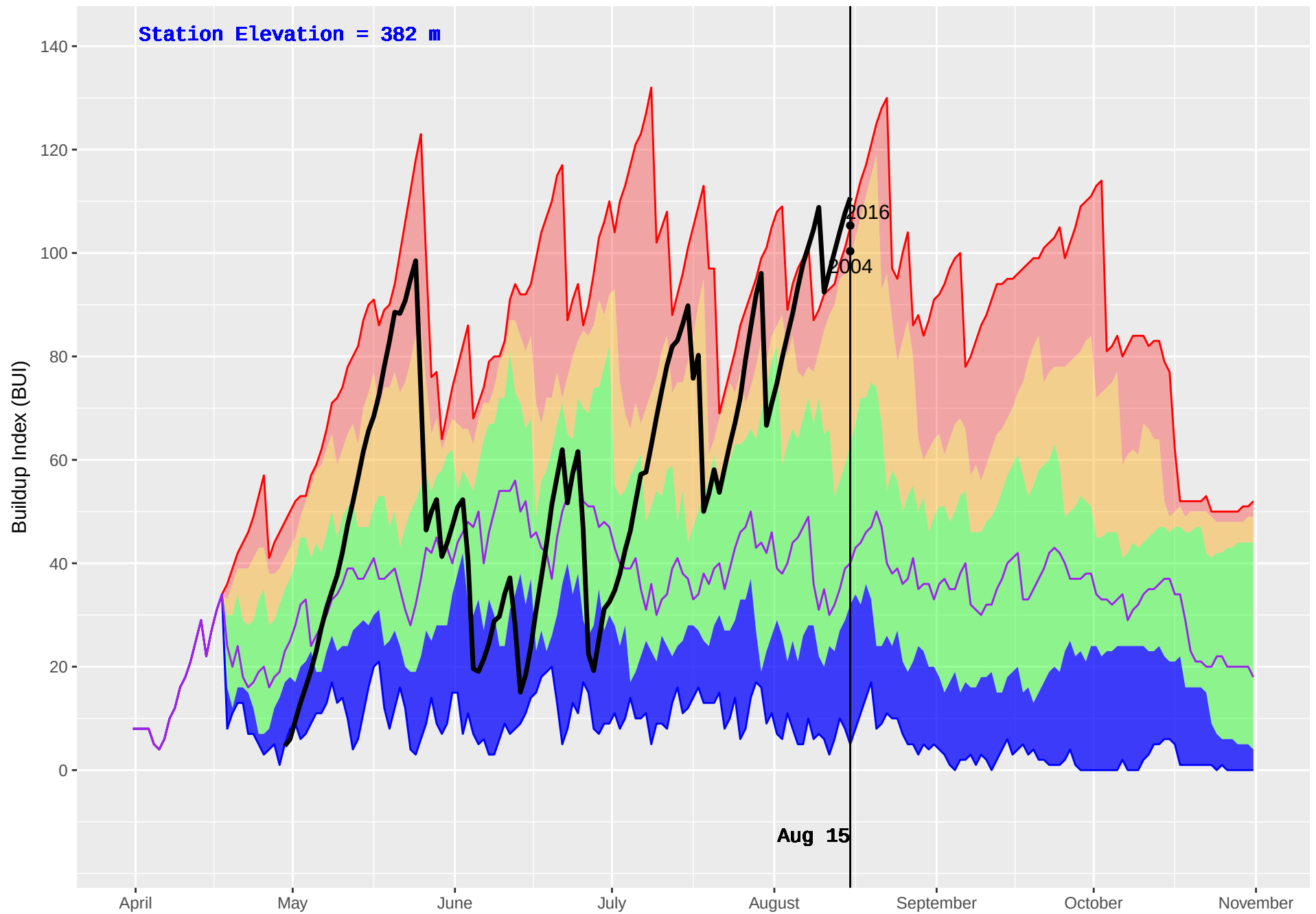
FORT NELSON FS (599) : Historical (1999–2016) and Current (2018) Daily Buildup Index (BUI)
