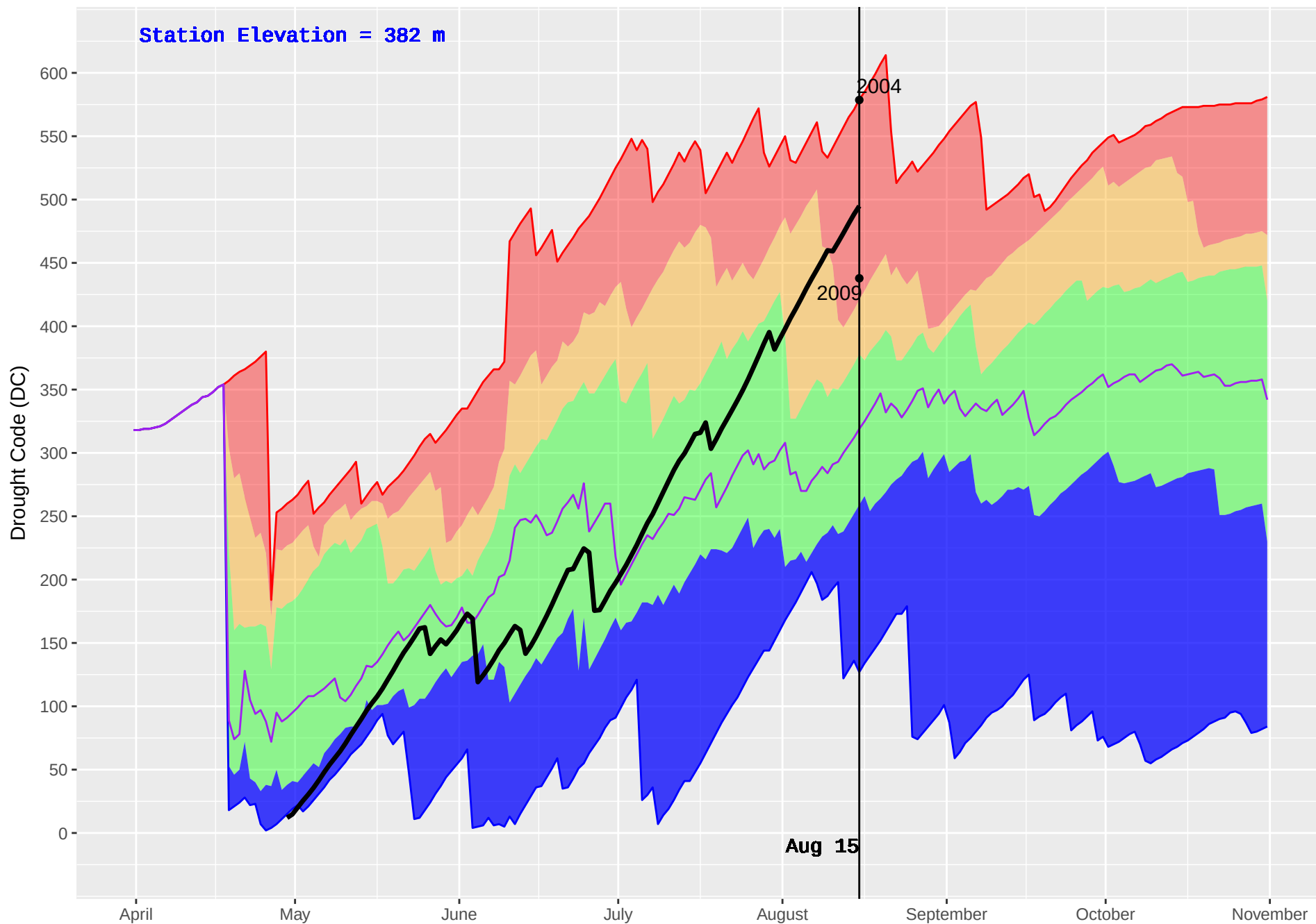
FORT NELSON FS (599) : Historical (1999–2016) and Current (2018) Daily Drought Code (DC)
